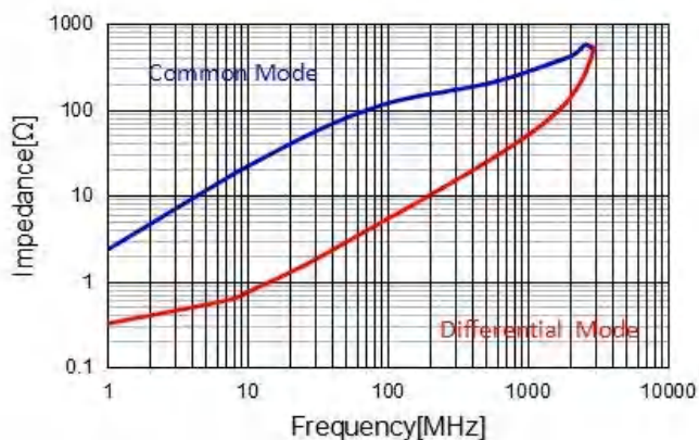
CMF3216S121T
