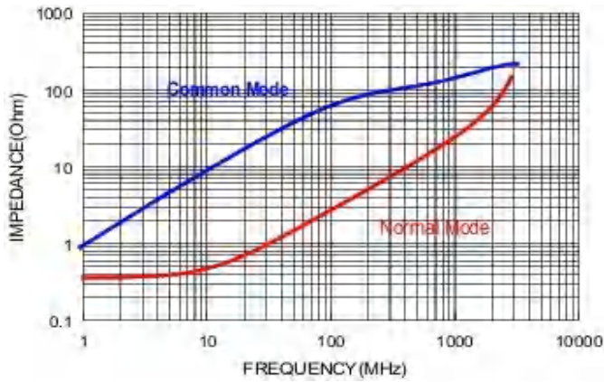
CMF1210S600T
