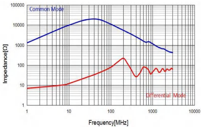
CMF3225L201T
