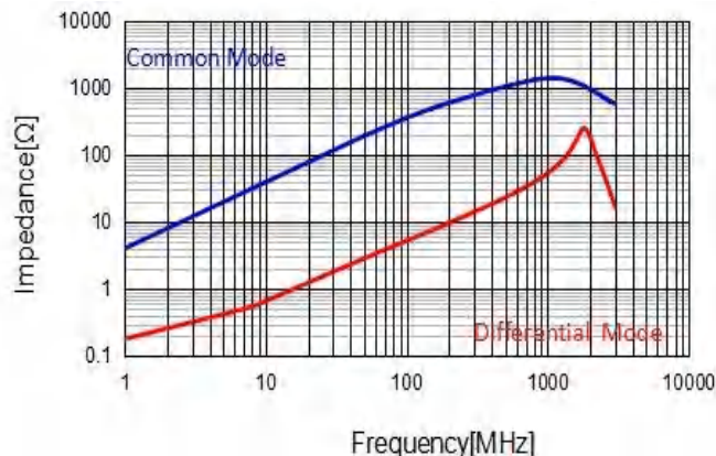
CMF2012S361T
