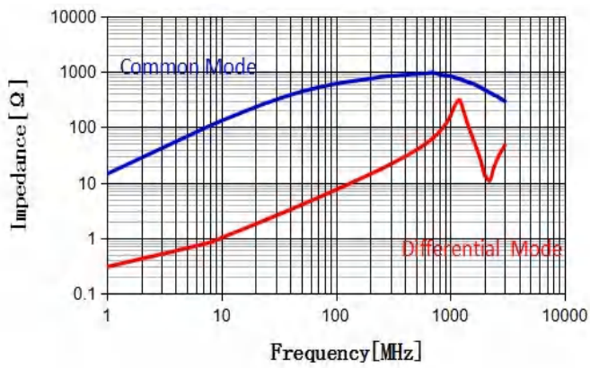
CMF3225S601T
