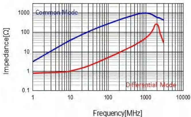
CMF2012S261T
