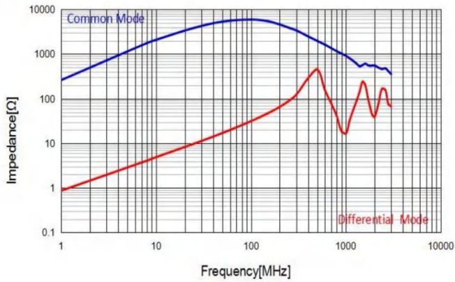
CMF3225L510T
