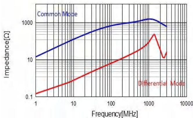
CMF2012S601T
