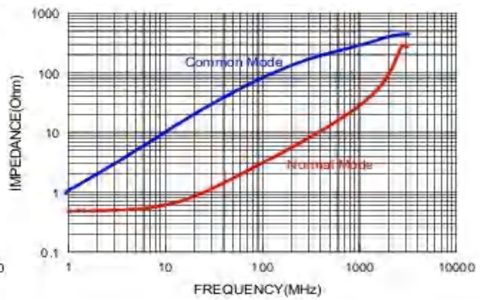
CMF1210S900T
