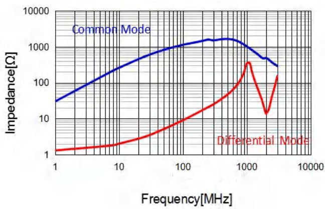
CMF3225S102T
