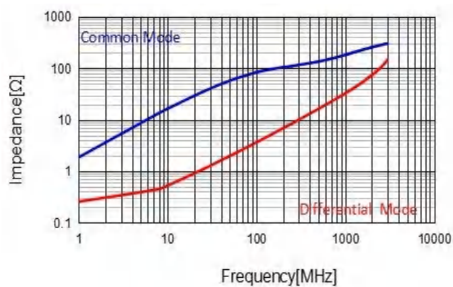
CMF2012S900T
