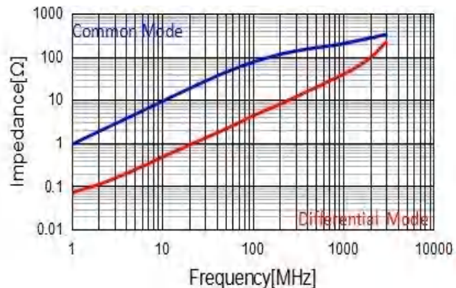
CMF2012S670T
