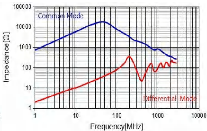
CMF4532L101T
