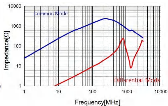
CMF4532S142T
