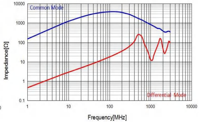
CMF3225L220T
