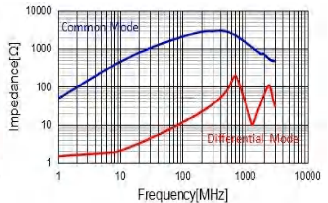
CMF3216S202T
