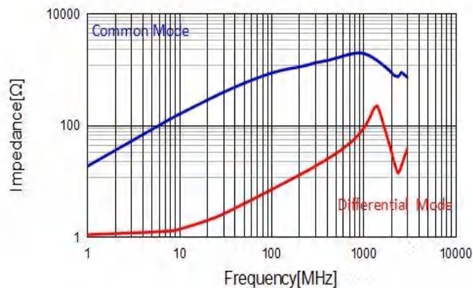
CMF2012S801T
