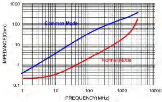
CMF1210S220T
