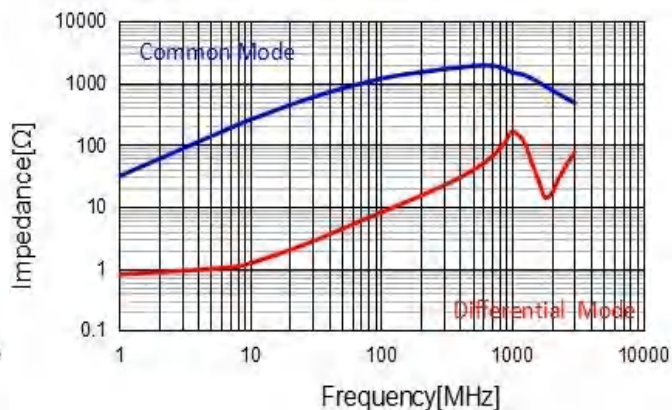
CMF2012S102T
