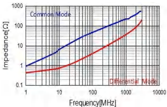
CMF2012S500T
