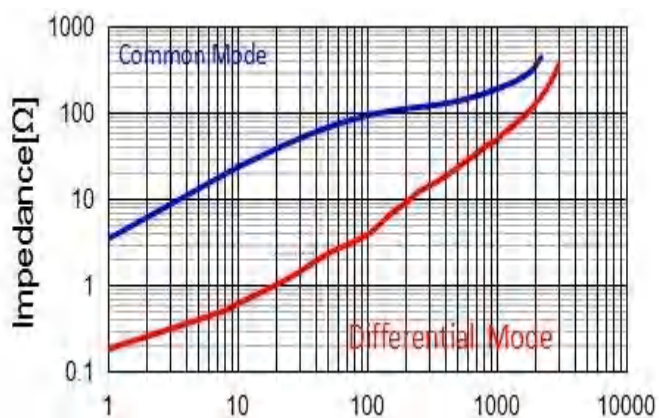
CMF4532S800T
