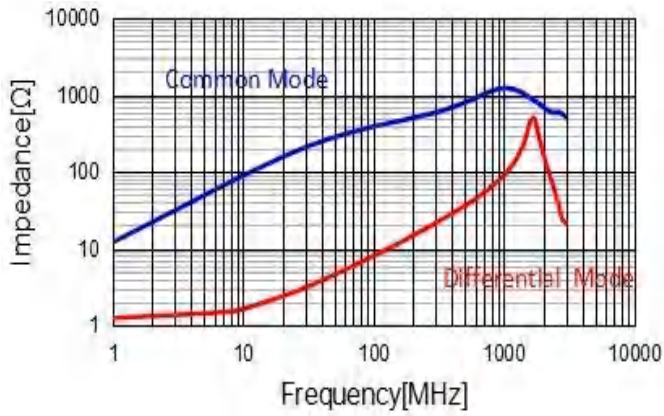
CMF3216S361T
