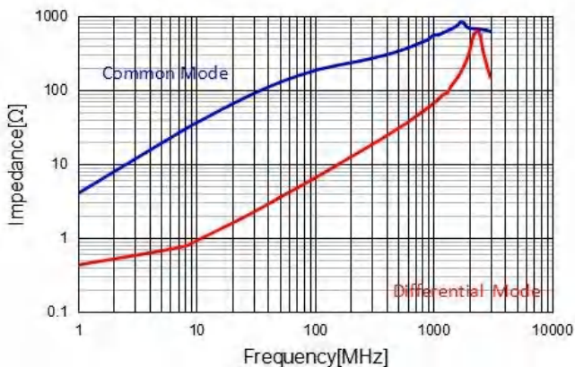
CMF3216S161T
