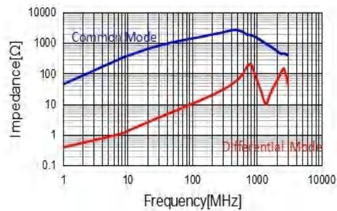
CMF3216S142T
