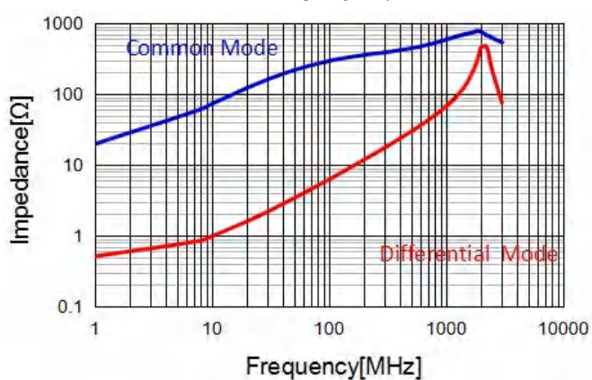
CMF3225S271T
