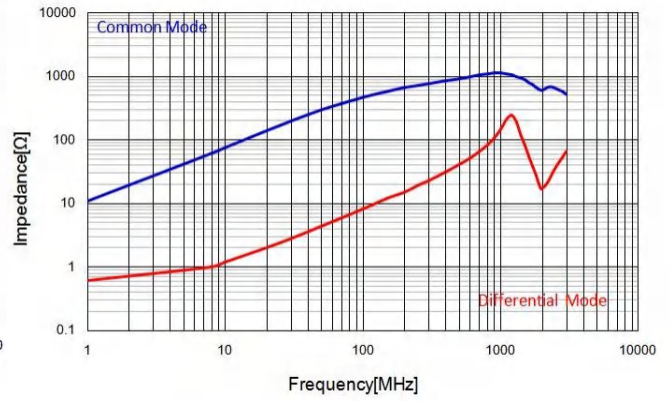
CMF2520S451T
