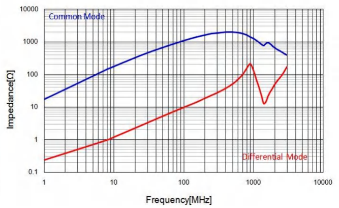
CMF2520S102T
