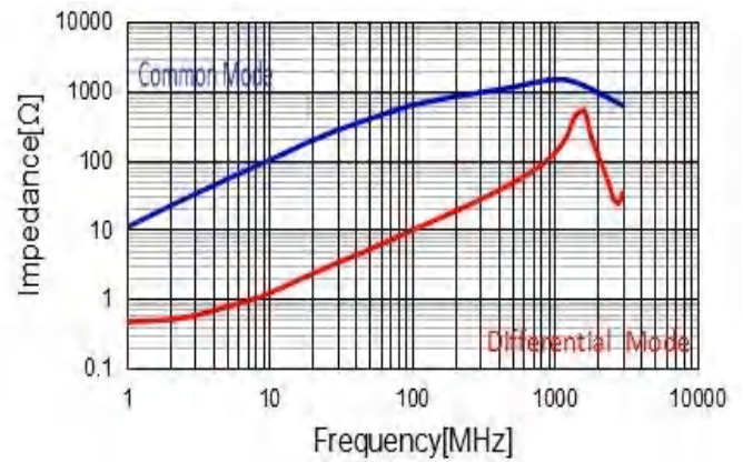
CMF3216S601T
