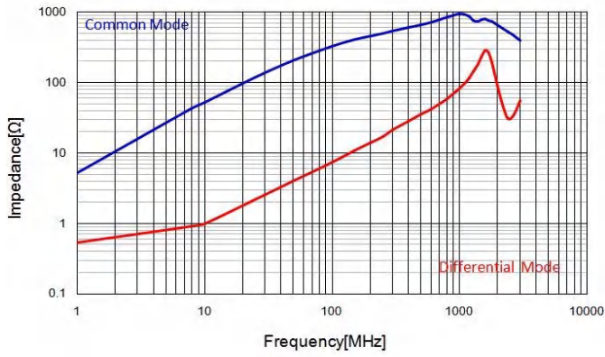
CMF2520S301T
