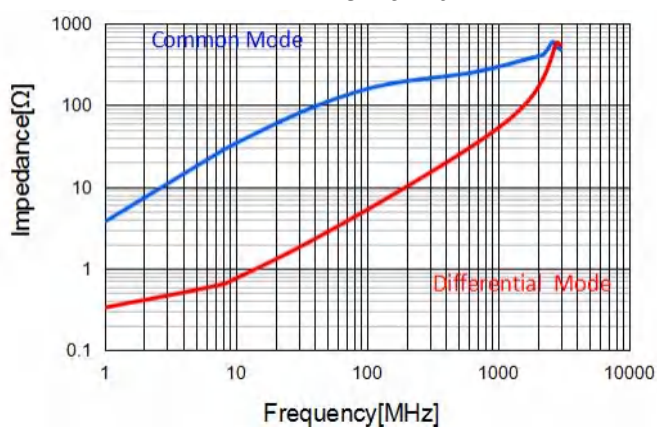
CMF3225S161T
