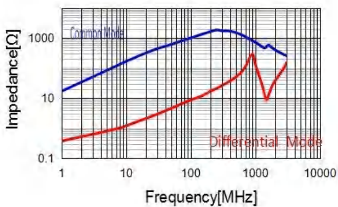
CMF4532S102T
