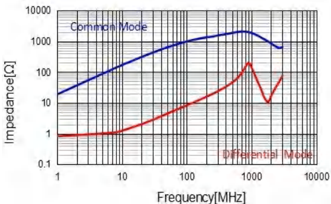
CMF2012S901T
