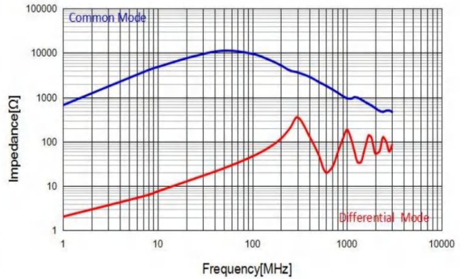
CMF3225L101T
