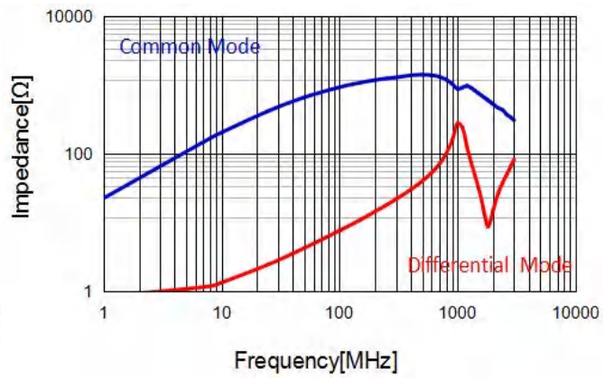
CMF3225S801T
