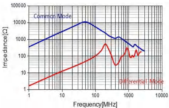
CMF4532L510T
