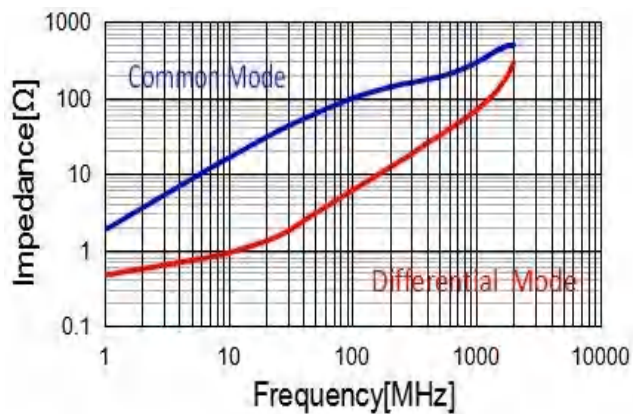
CMF4532S900T
