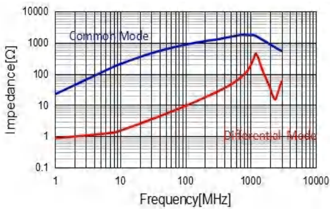
CMF3216S801T
