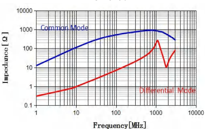
CMF3225S501T
