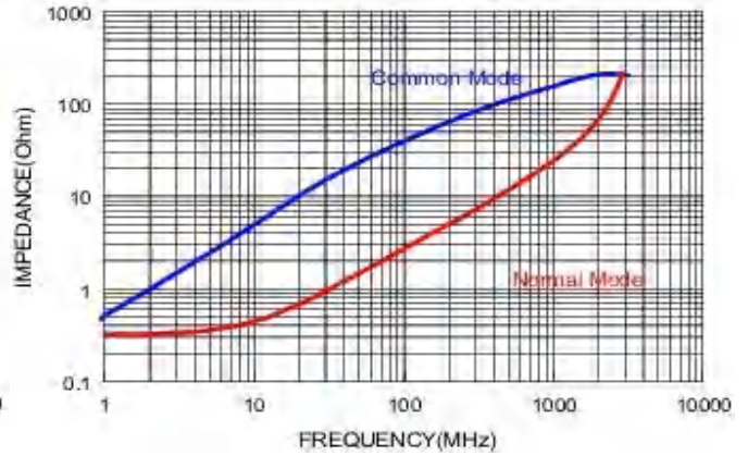
CMF1210S500T
