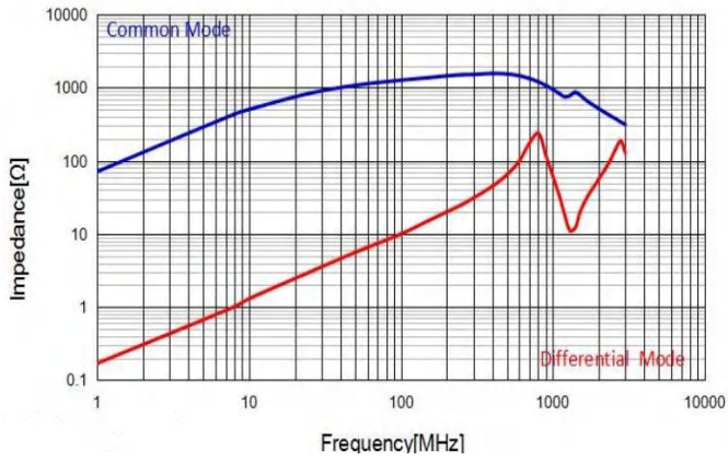
CMF3225L110T
