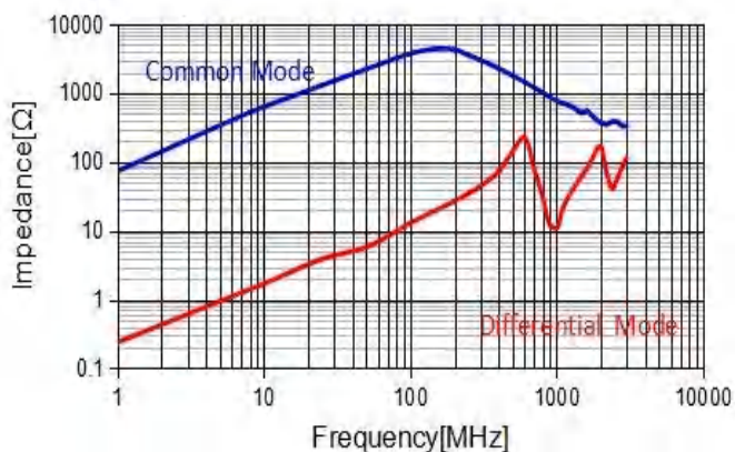
CMF4532L110T
