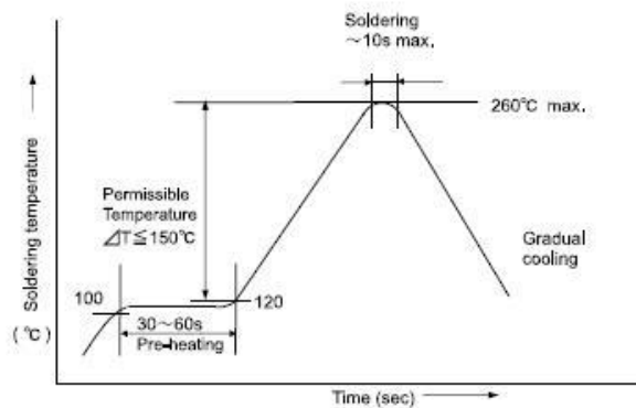
Flow soldering recommended condition
